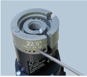
Grinding electrodes: 4 different angles and 6 different electrode sizes
